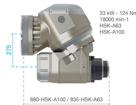
Cabezal 30° con electromandrino 30° head with electros spindle
